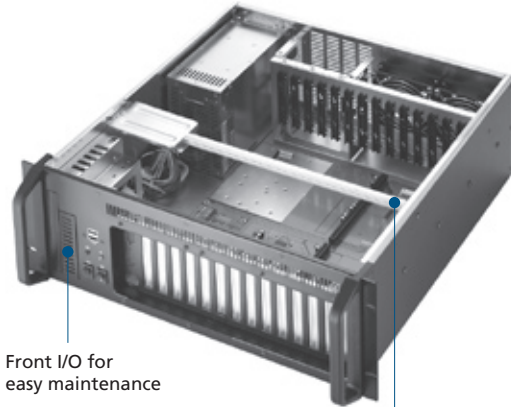
Flexible hold-on clamp bar with adjustable clips to secure add-on card in different height
