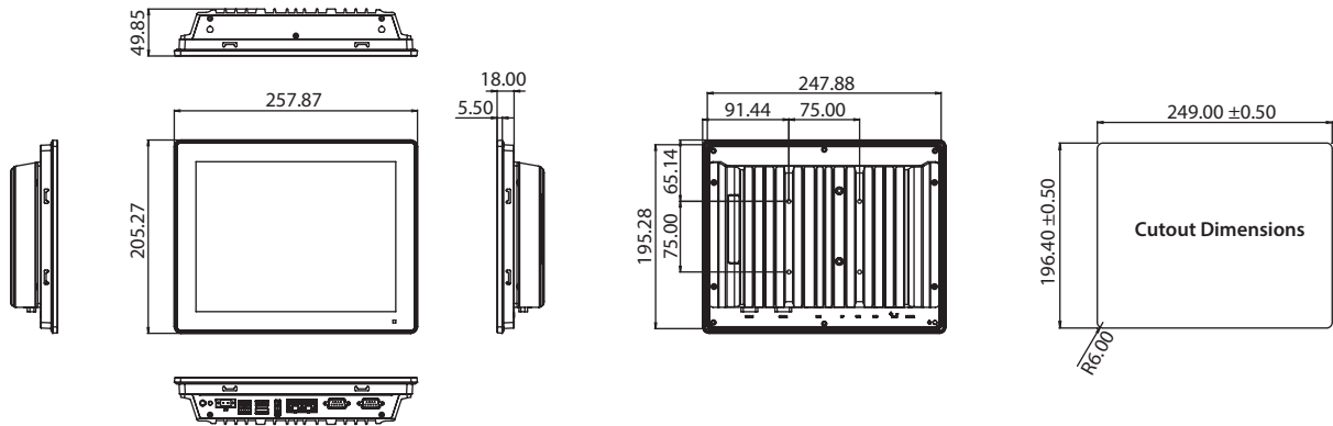
Panel Cutout Dimensions: 249 x 196.4 mm (9.81 x 7.74 in)
