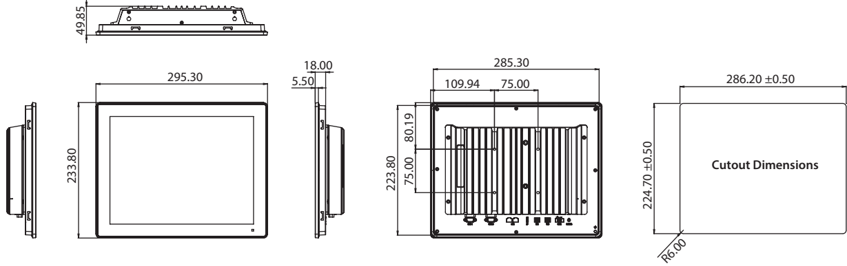
Panel Cutout Dimensions: 286.2 x 224.7 mm (11.27 x 8.85 in)
